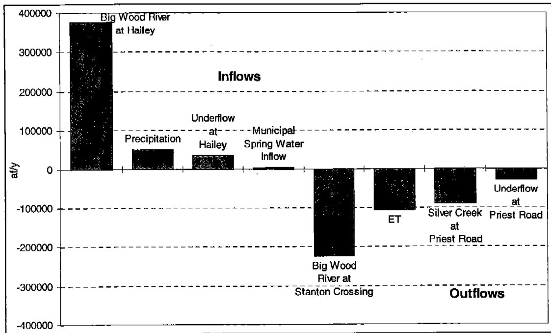
Figure 17. Big Wood River -- Silver Creek Aquifer System Surface and Ground Water Budget
