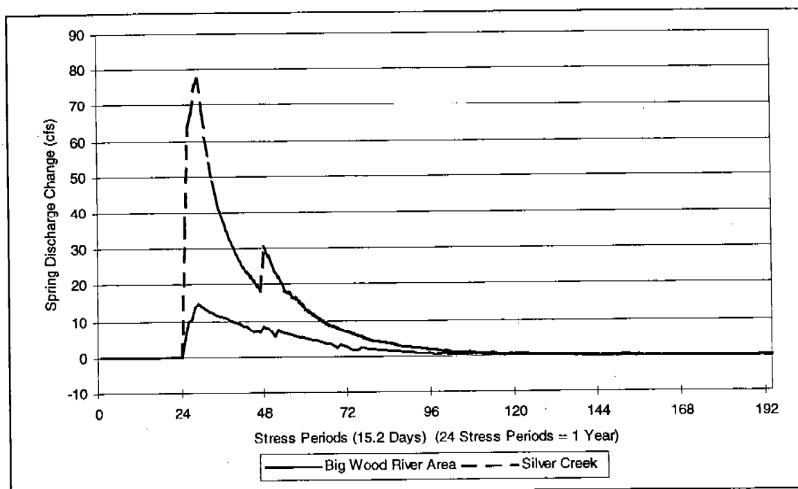
Figure 43. Reference Scenario vs Recharge with Maximum Excess Big Wood River Flows Scenario Spring Flows
