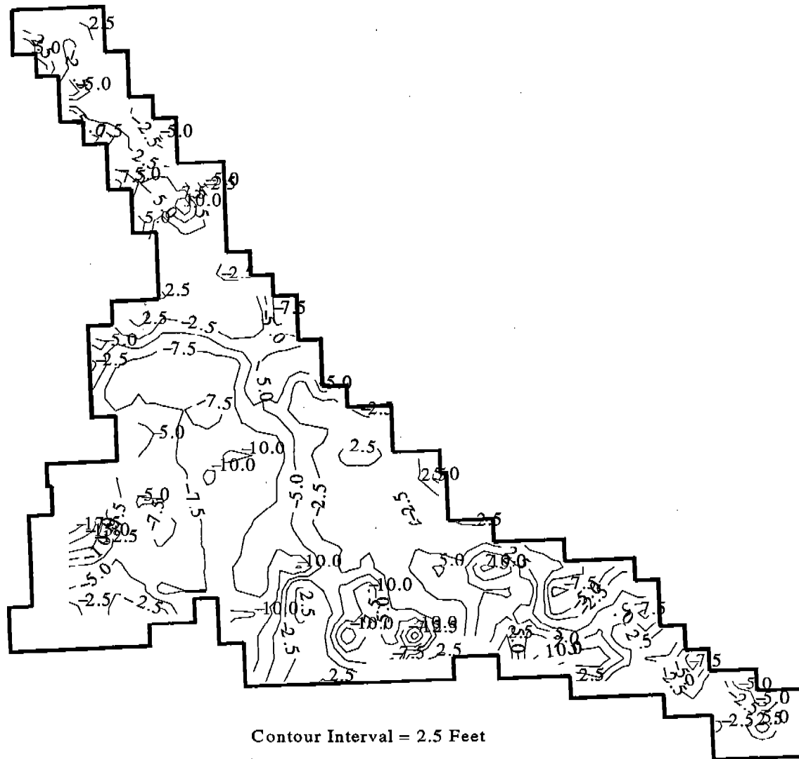
Figure 24. Differences between Estimated and Simulated Water Surface for Stress Period 8 in Layer 3
