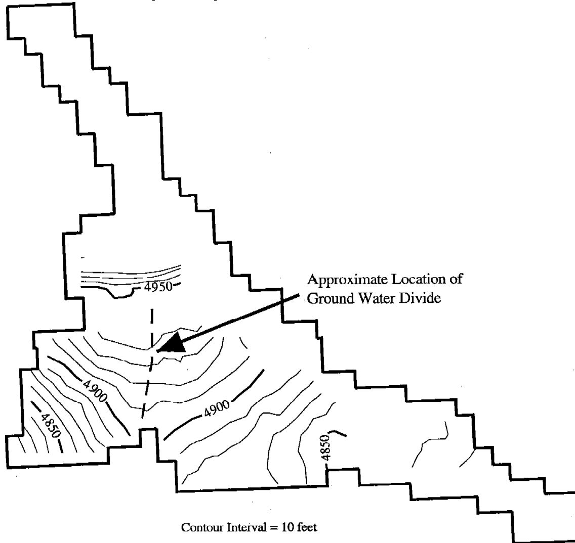
Figure 8. Layer 1 Spring 1993 Estimated Water Surface Elevation
