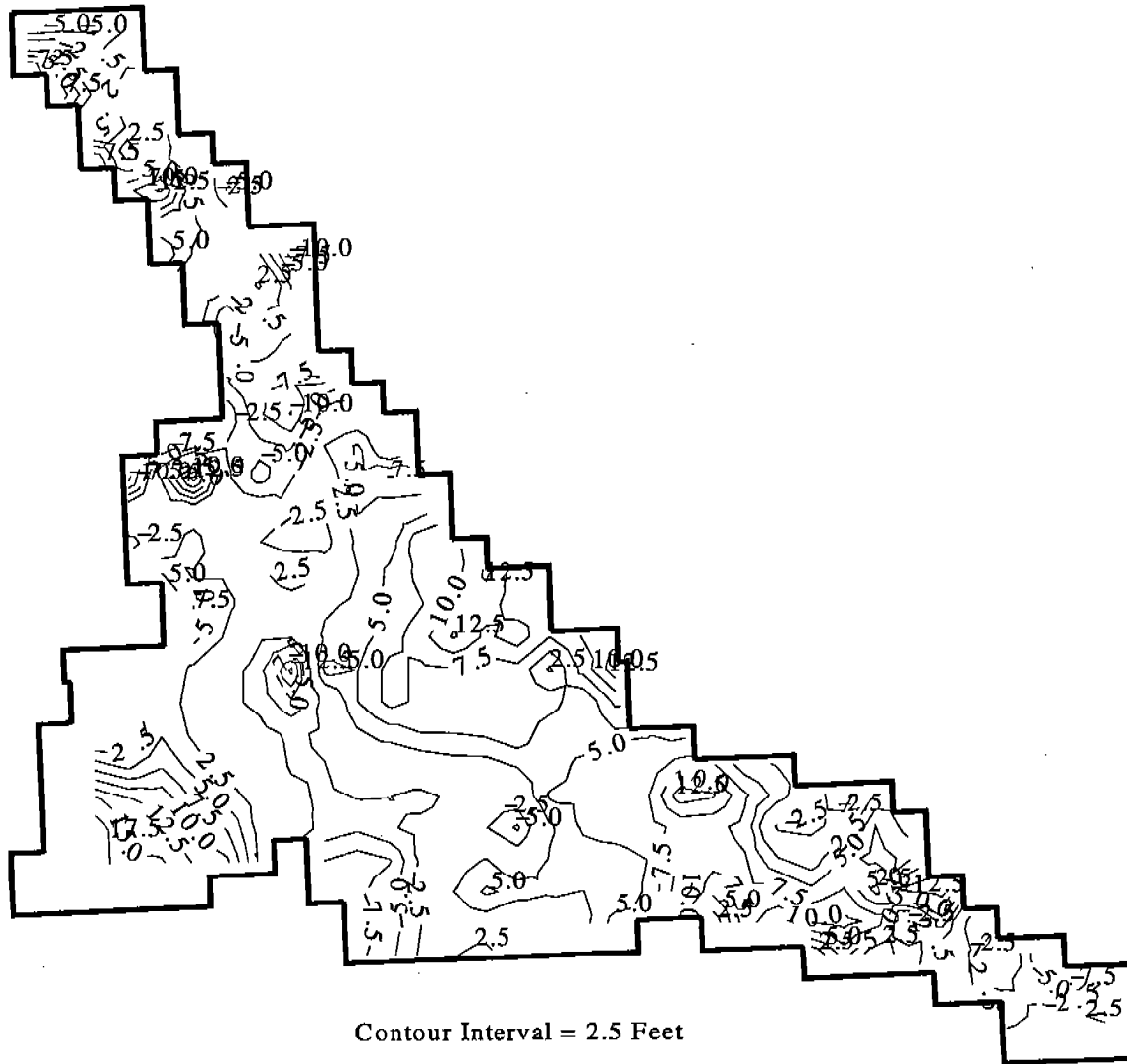
Figure 28. Differences between Estimated and Simulated Water Surface for Stress Period 24 in Layer 3
