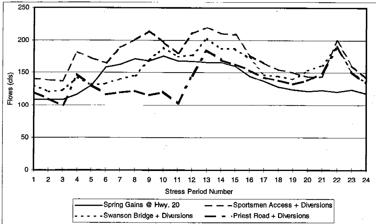
Figure 22. Silver Creek Stream Flow and Diversions.
