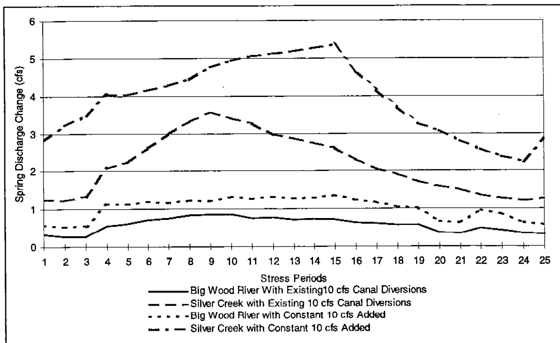
Figure 44. Reference Scenario vs Recharge with Canal Diversion Scenario Spring Flows
