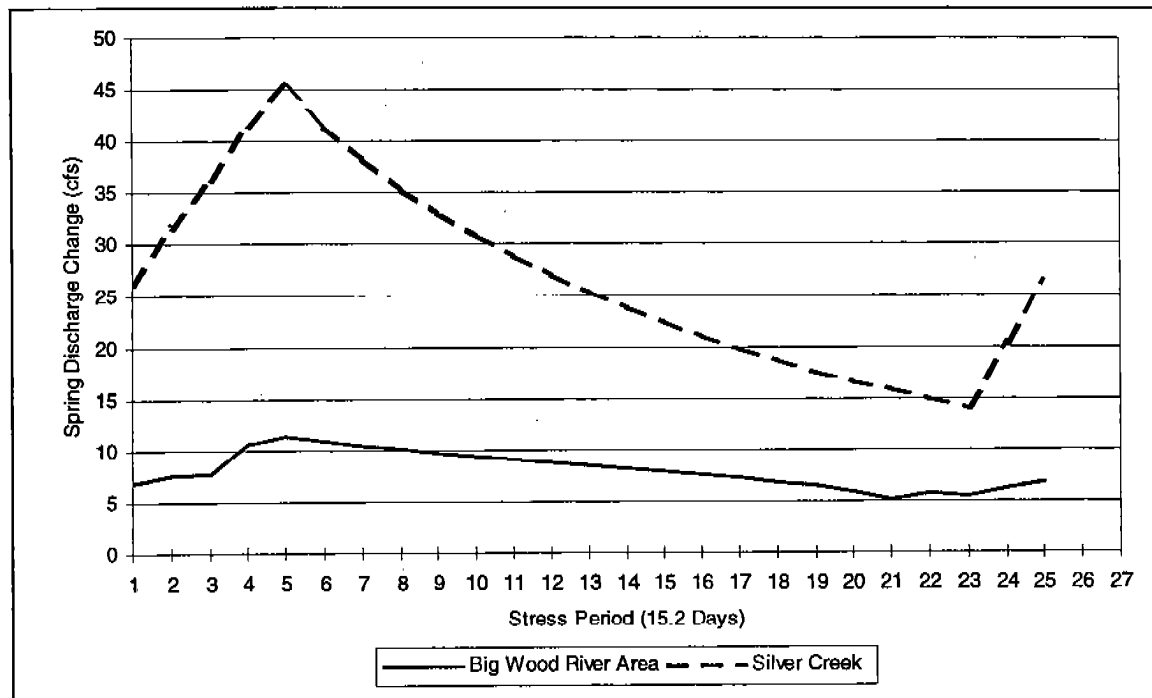
Figure 42. Reference Scenario vs Recharge with Excess Yearly Average Big Wood River Flows Scenario Spring Flows
