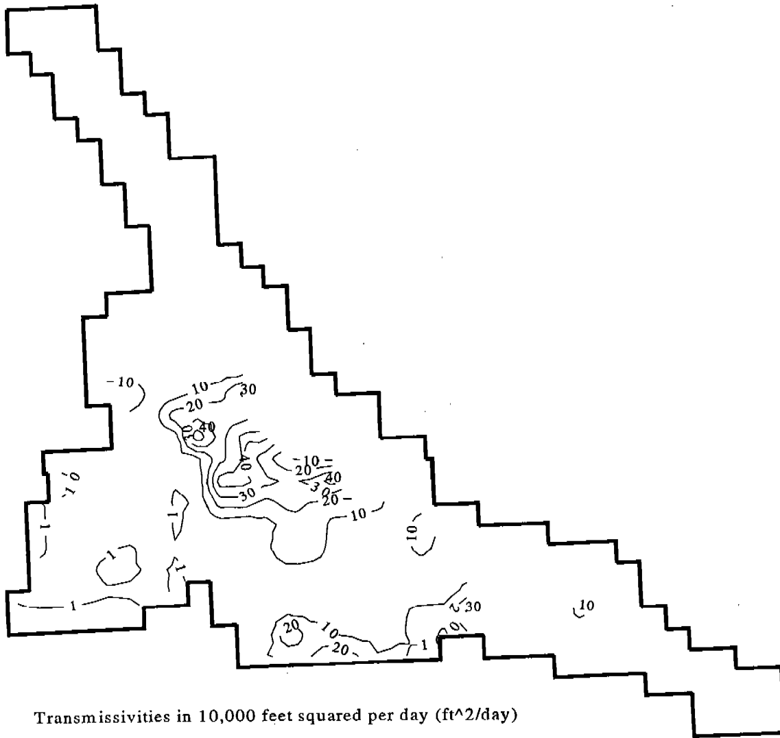
Figure 30. Layer 1 Transmissivities
