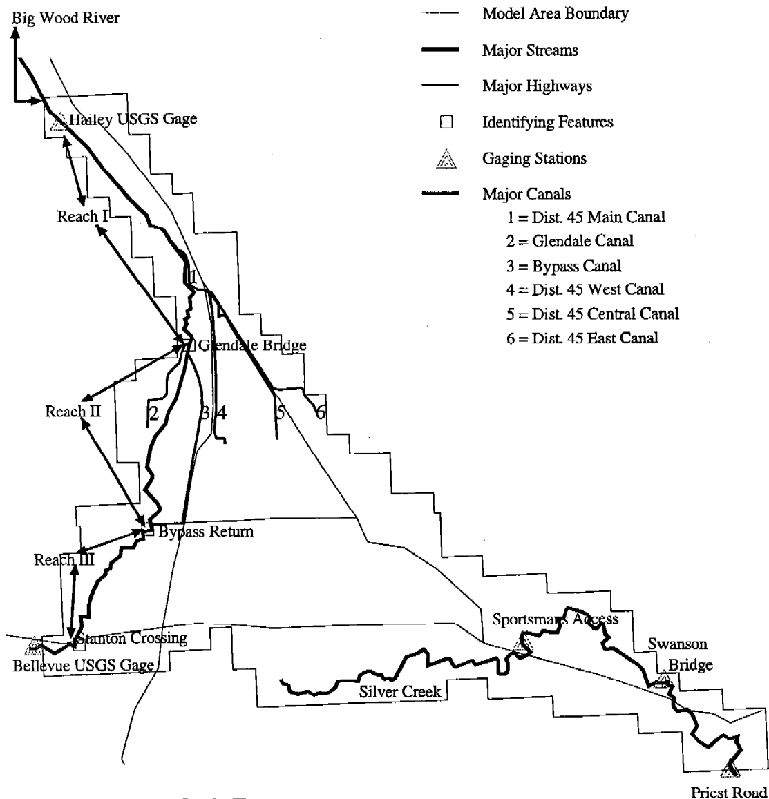
Figure 4. Hydrologic Features
