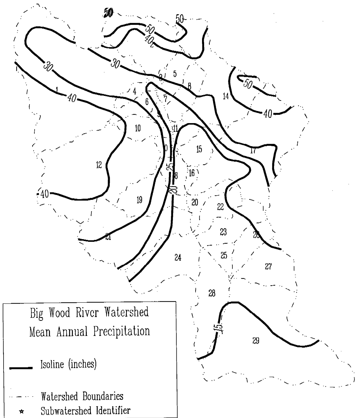
Figure 46. Mean Annual Precipitation, 1961-90
