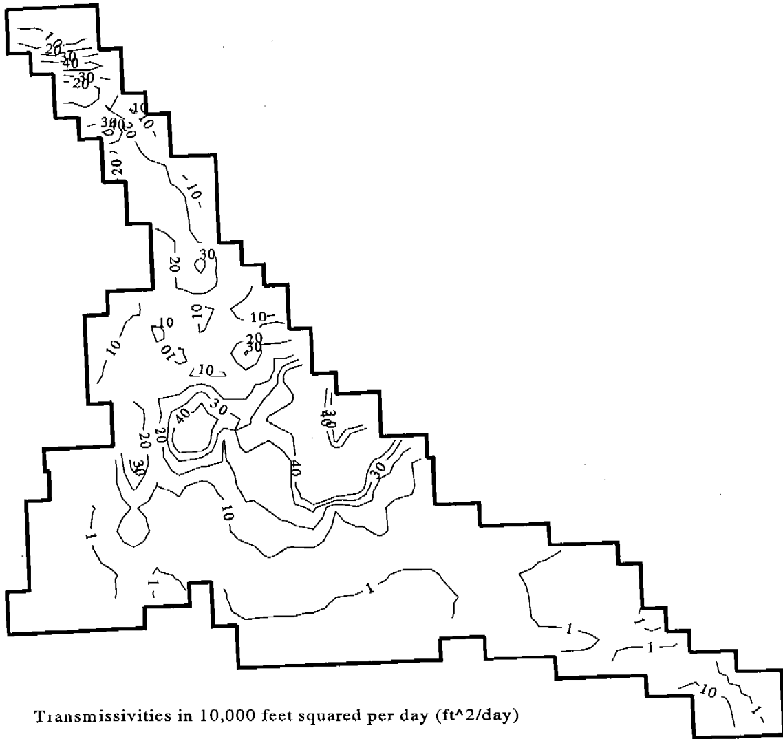
Figure 31. Layer 3 Transmissivities
