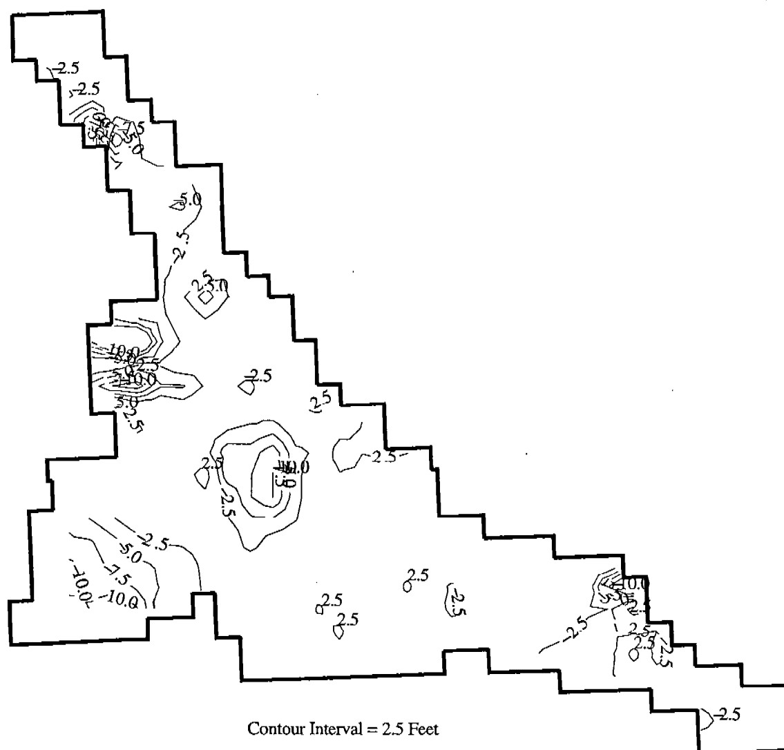
Figure 15. Layer 3 Difference Between Spring 1993 and Spring 1994
