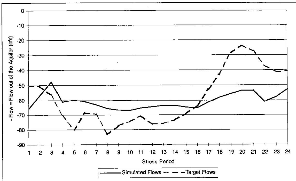
Figure 32. 1993 Target vs Simulated Spring Flows for Big Wood River Area
