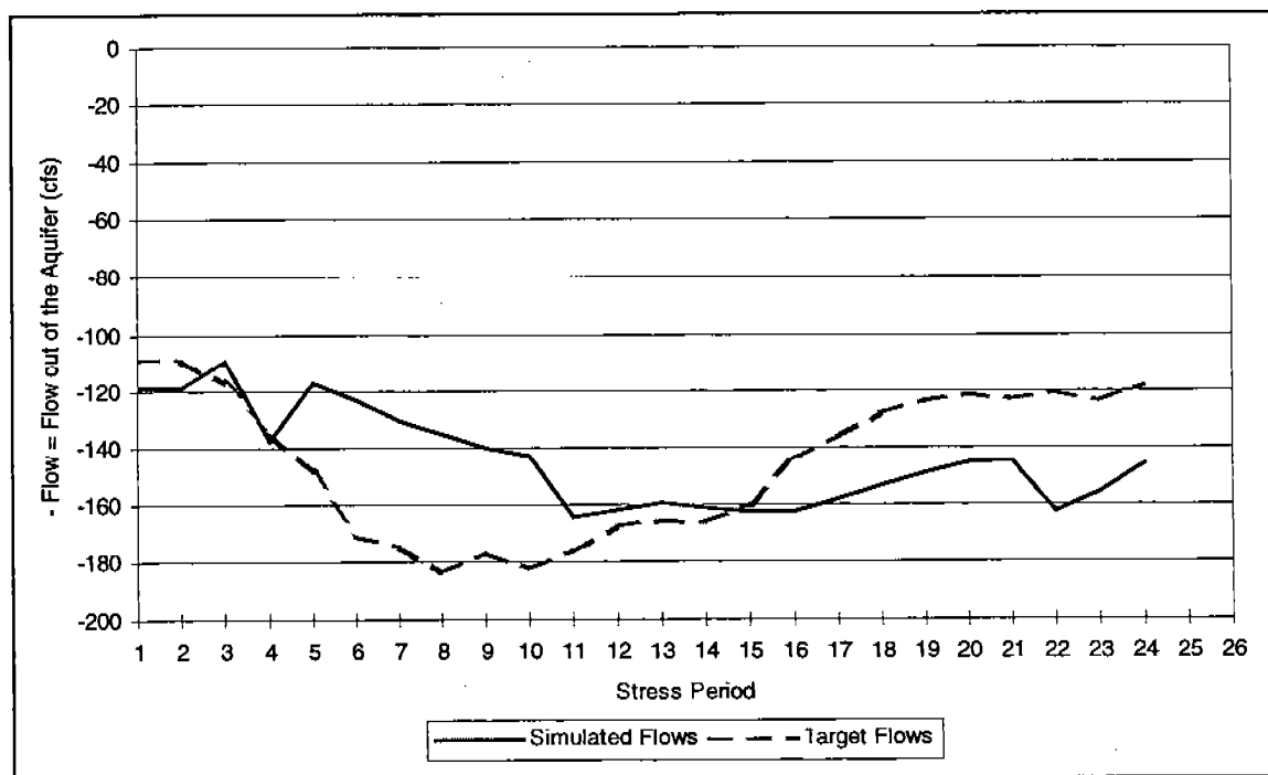
Figure 33. 1993 Target vs Simulated Flows for Springs Tributary to Silver Creek
