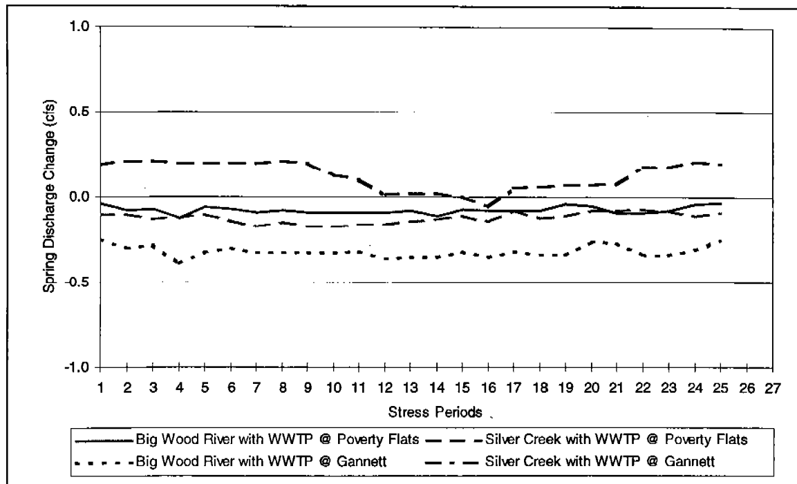
Figure 41. Reference Scenario vs Combined Waste Water Treatment Plant Scenario Spring Flows
