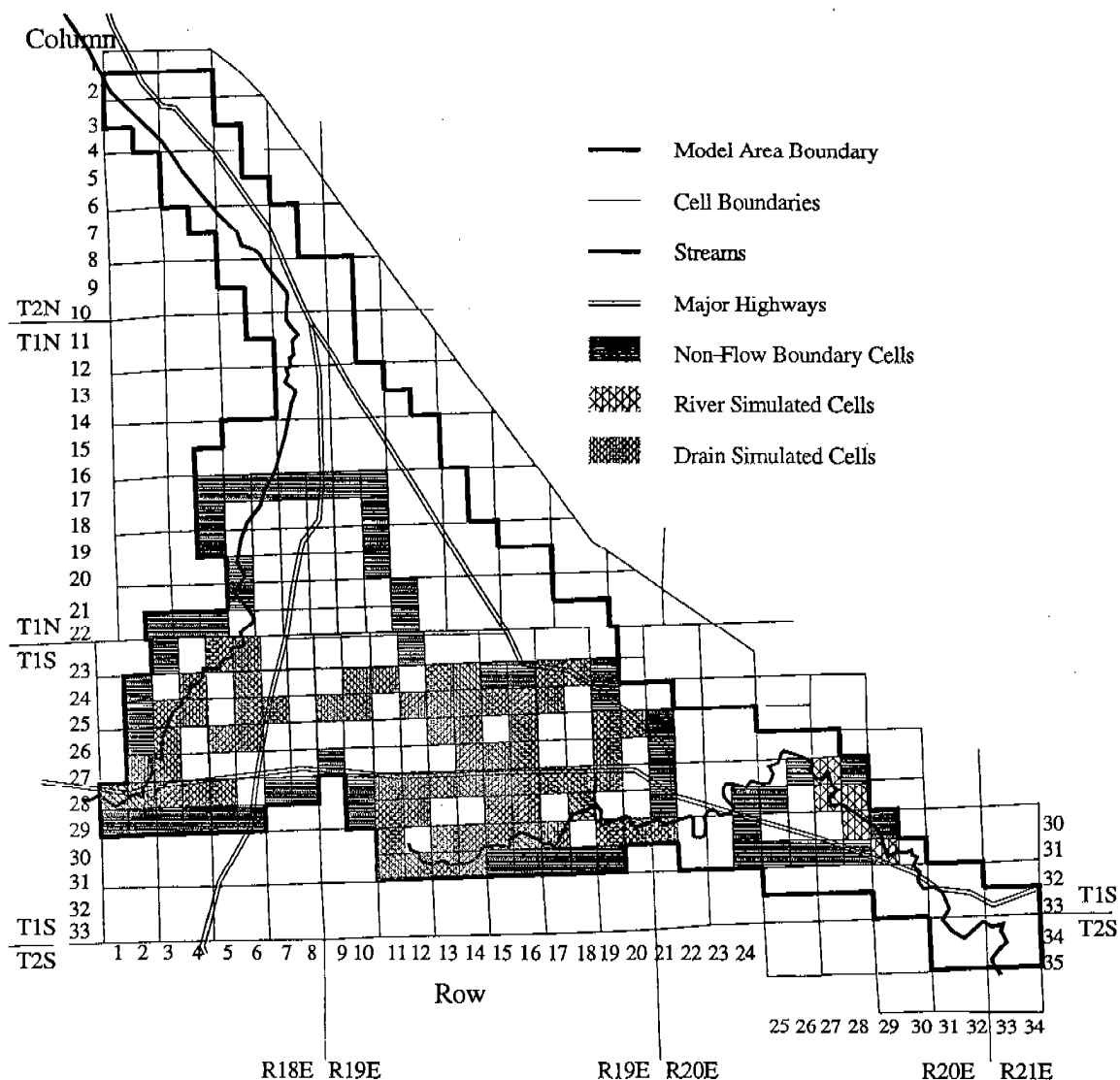
Figure 7. Boundary Conditions and River and Drain Simulated Cells, Layer 1
