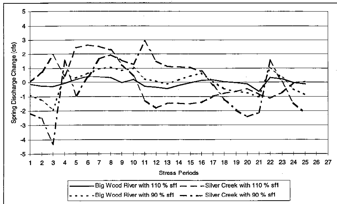
Figure 38. Flow Sensitivity to Changes in Specific Yield Storage Coefficient
