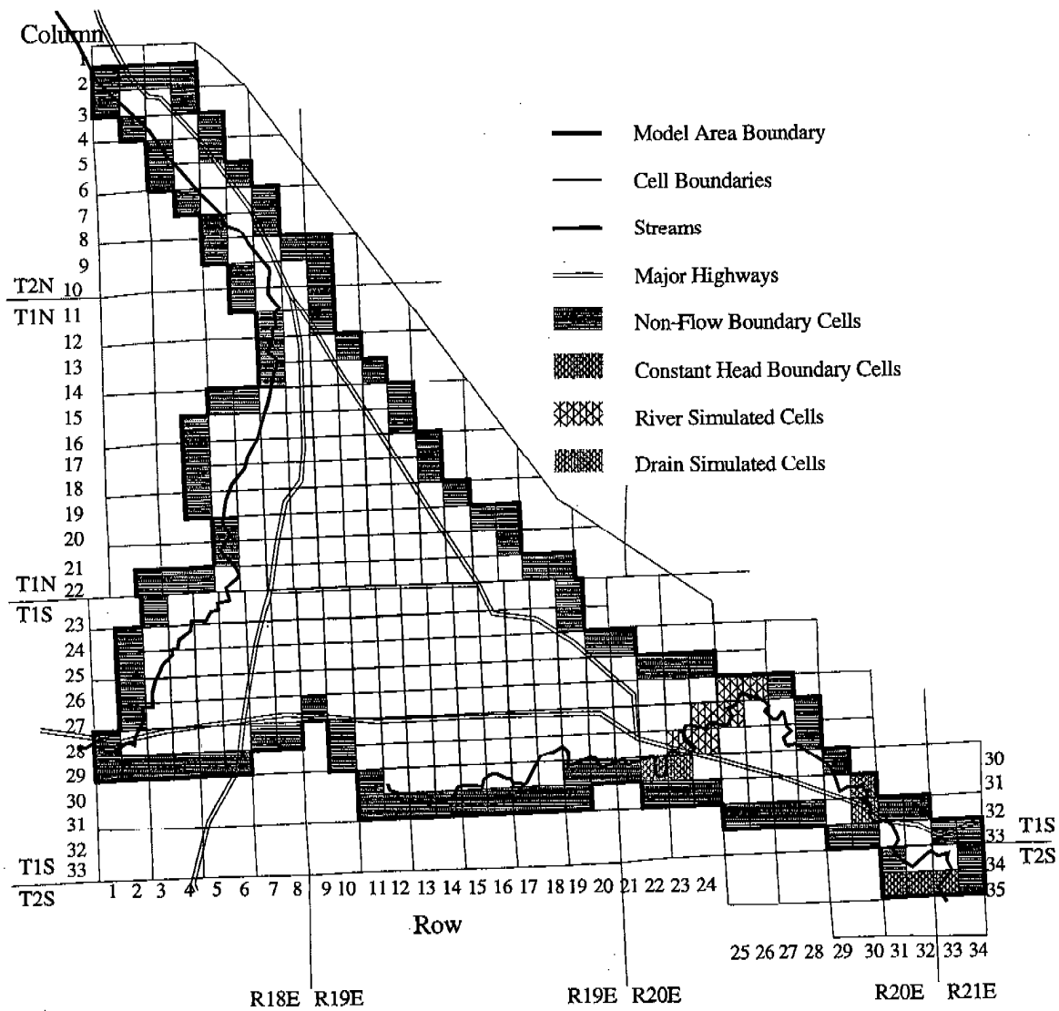
Figure 6. Boundary Conditions and River Simulated Cells, Layer 3
