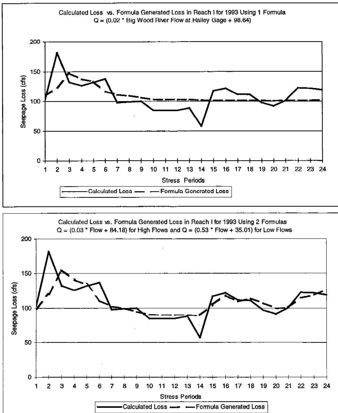
Figure 35. Formulas to Calculate Big Wood River Seepage Losses.
