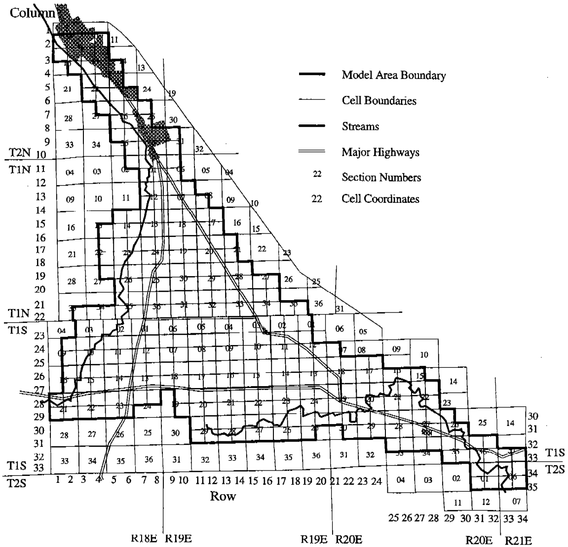
Figure 5. Ground Water Model Grid and Coordinates
