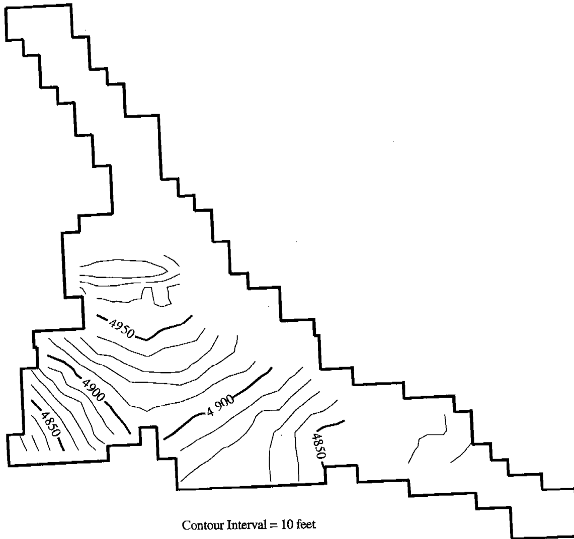
Figure 10. Layer 1 Summer 1993 Estimated Water Surface Elevation
