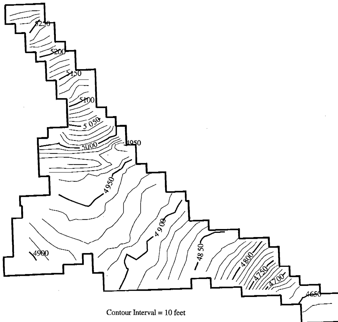
Figure 11. Layer 3 Summer 1993 Estimated Water Surface Elevation
