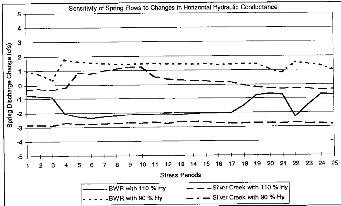
Figure 36. Flow Sensitivity to Changes in Hydraulic Conductivity.
