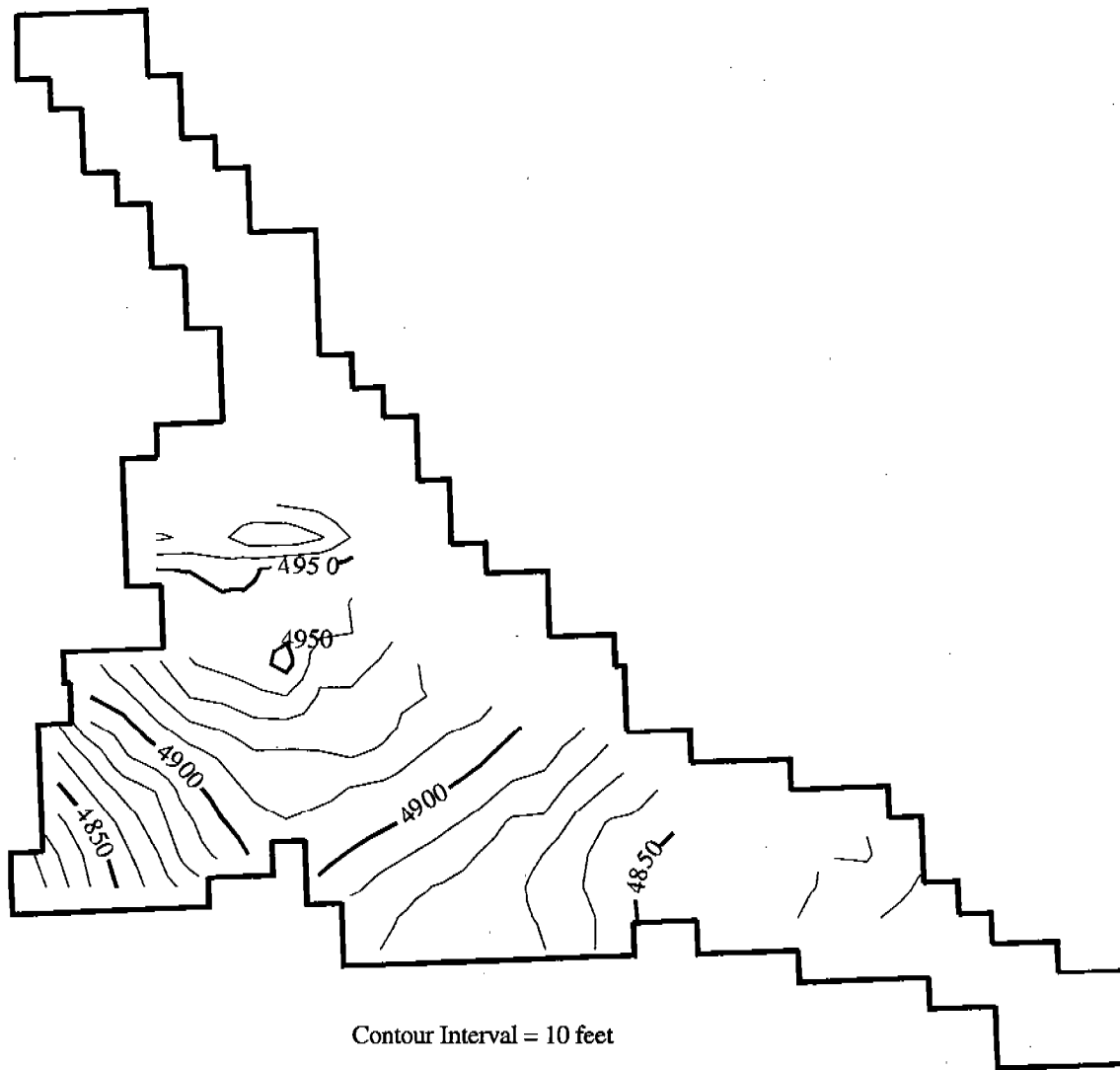
Figure 12. Layer 1 Spring 1994 Estimated Water Surface Elevation
