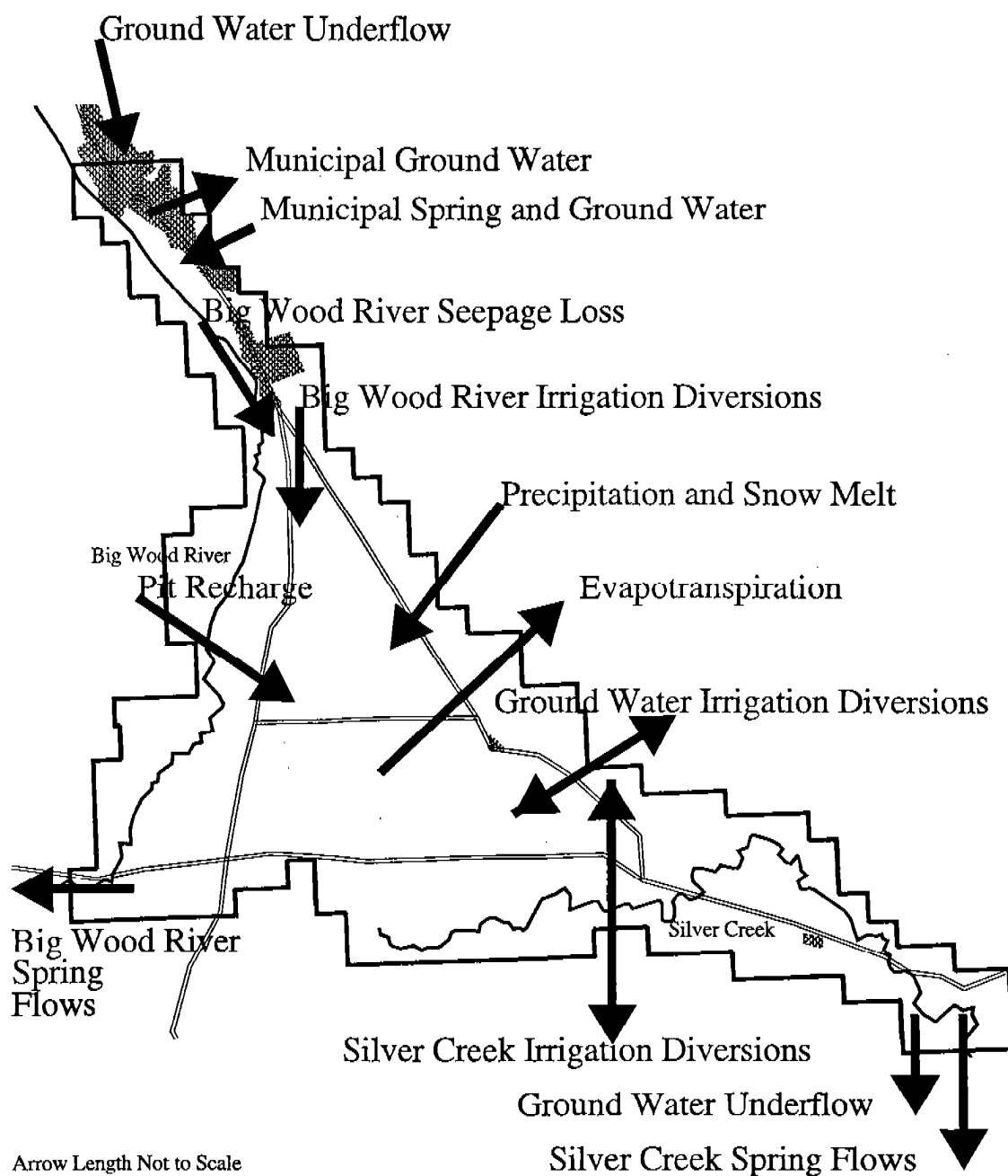
Figure 18. Conceptual Big Wood River – Silver Creek Aquifer System Ground Water Budget
