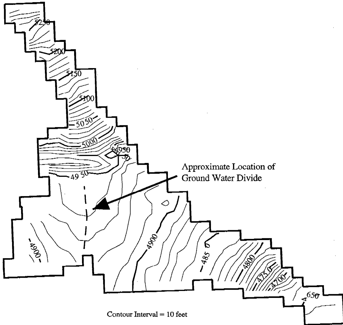
Figure 9. Layer 3 Spring 1993 Estimated Water Surface Elevation
