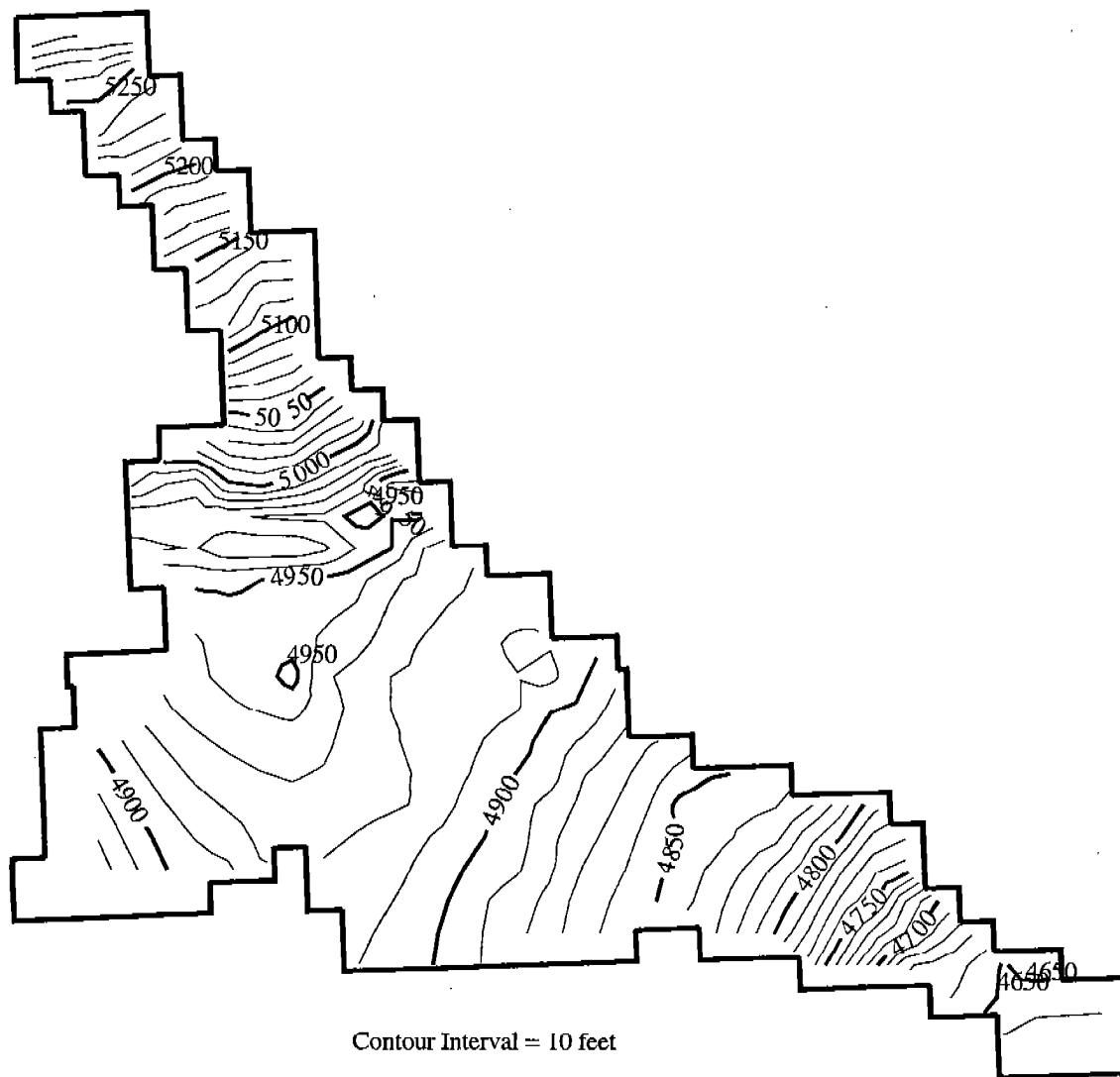
Figure 13. Layer 3 Spring 1994 Estimated Water Surface Elevation
