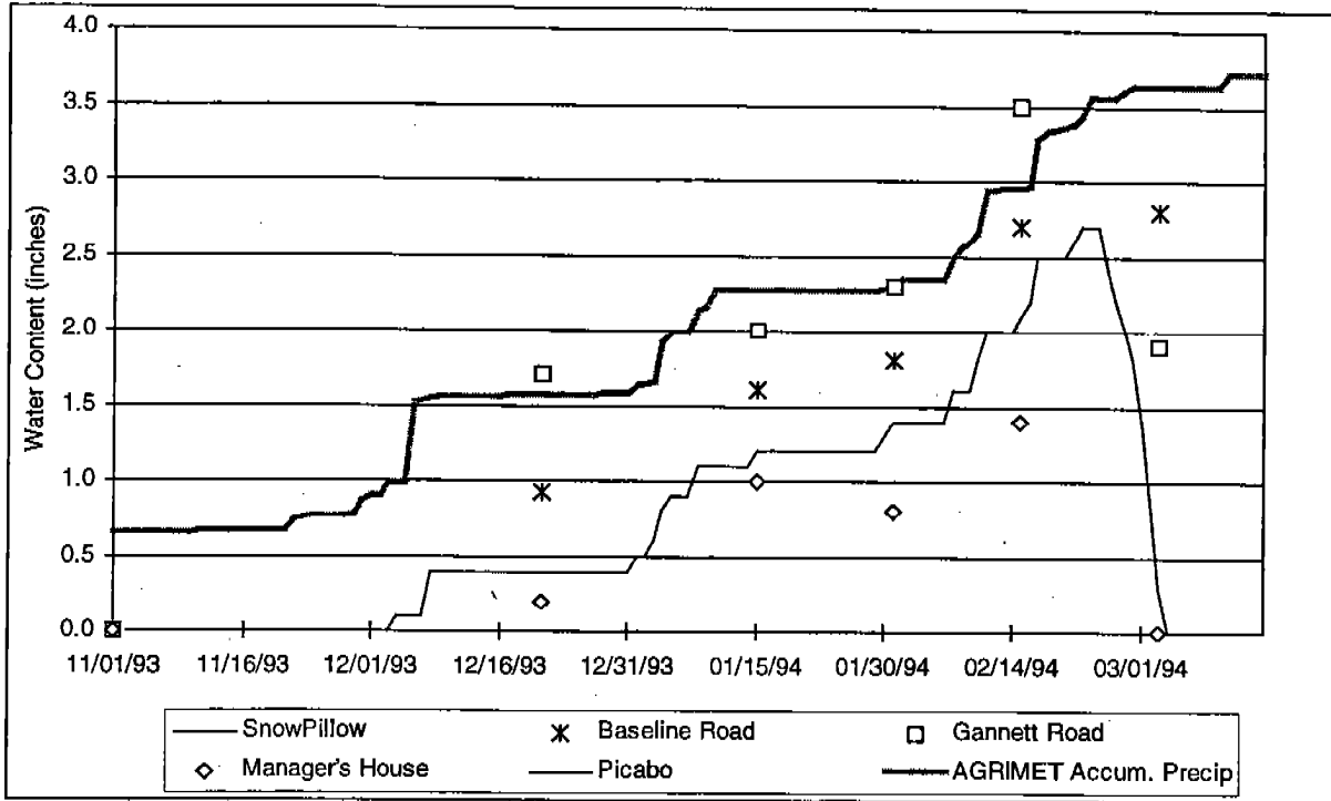
Figure 21. Snow Course-Snow Pillow Accumulated Snow Pack
