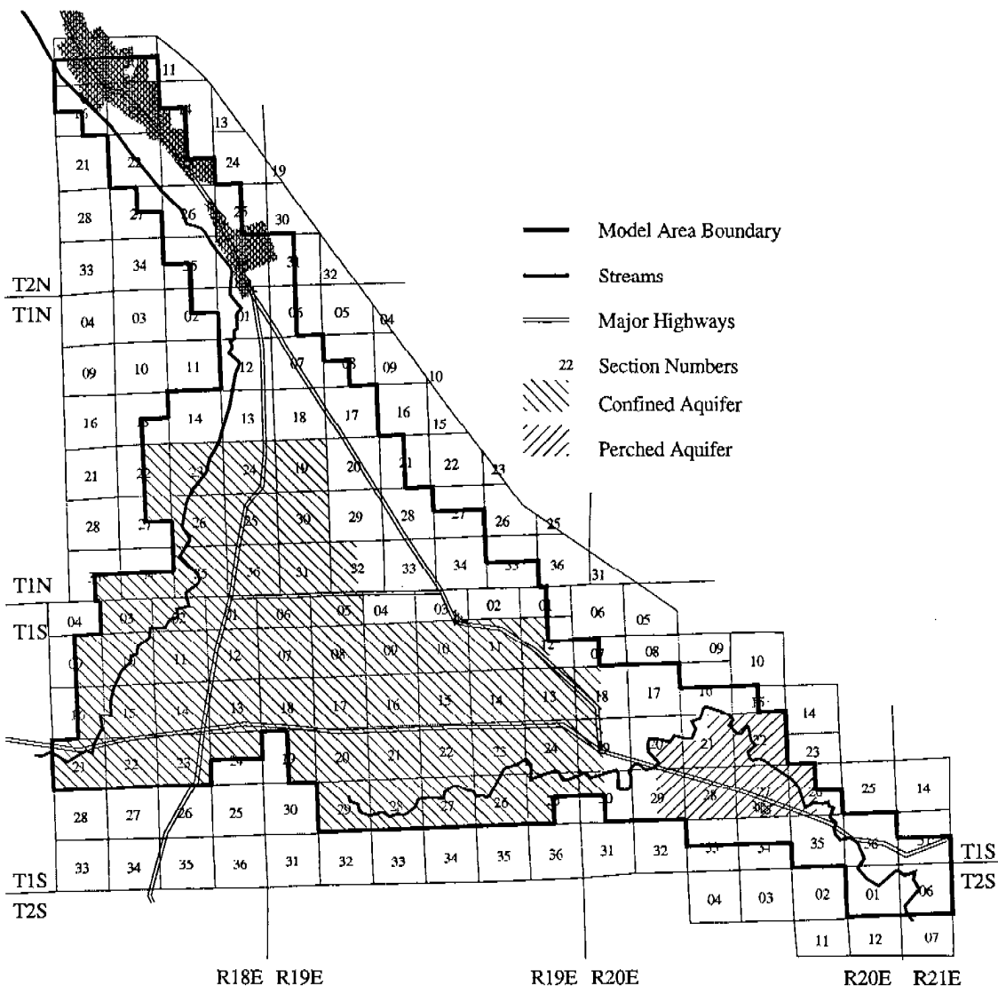
Figure 3. Approximate Extent of Aquifers
