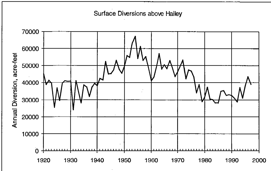
Figure 49. Upper Valley Historical Surface Diversions, 1921-97
