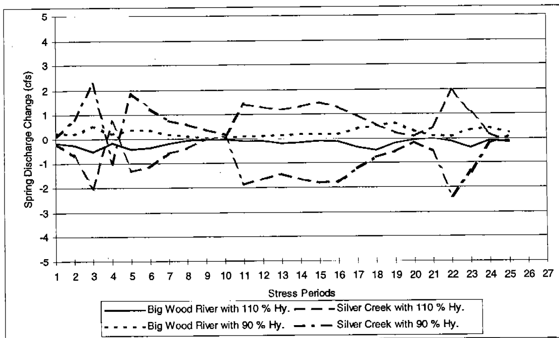
Figure 37. Flow Sensitivity to Changes in Drain and River Hydraulic Conductivity
