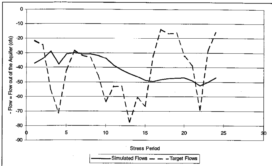
Figure 34. 1993 Target vs Simulated Flows for Silver Creek above Swanson Bridge
