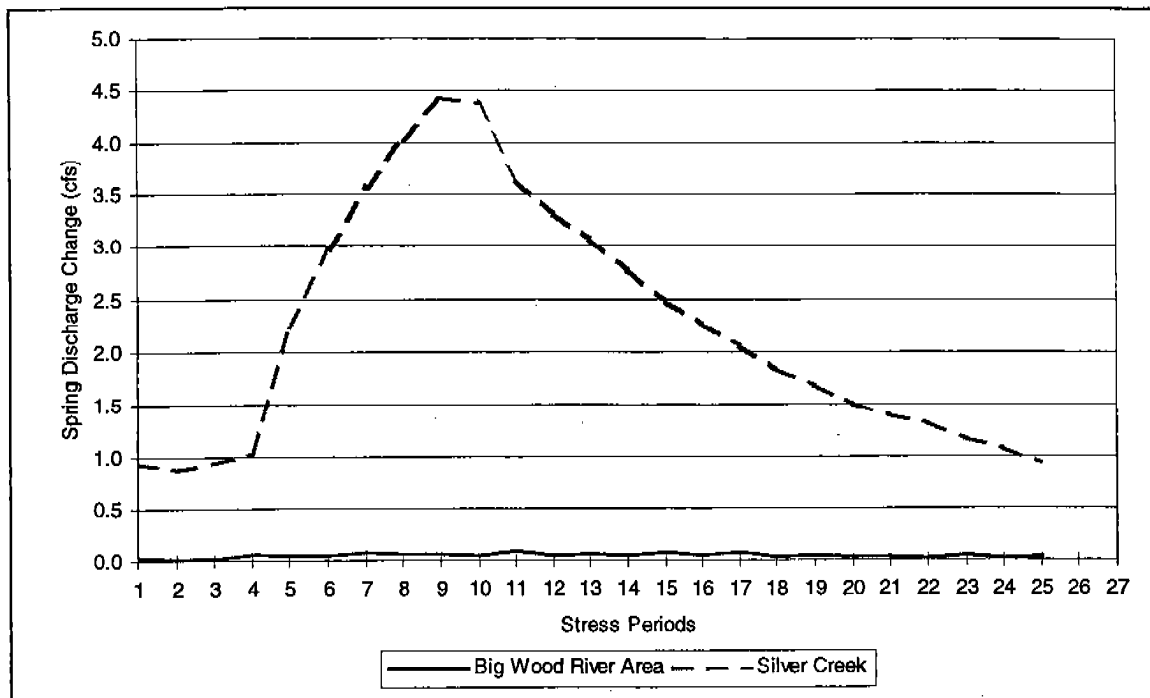
Figure 40. Reference Scenario vs Selected Well Removal Scenario Spring Flows
