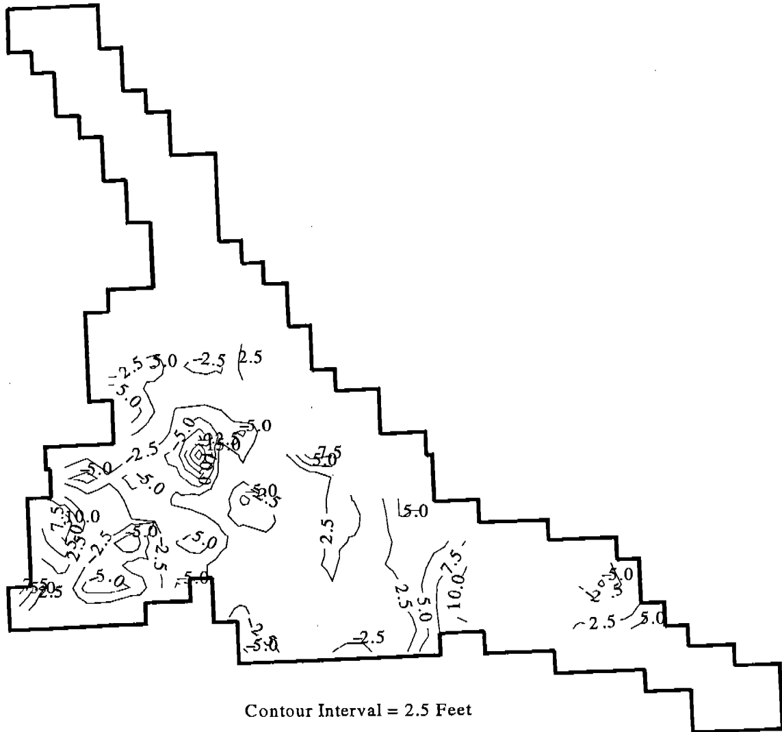
Figure 27. Differences between Estimated and Simulated Water Surface for Stress Period 24 in Layer 1
