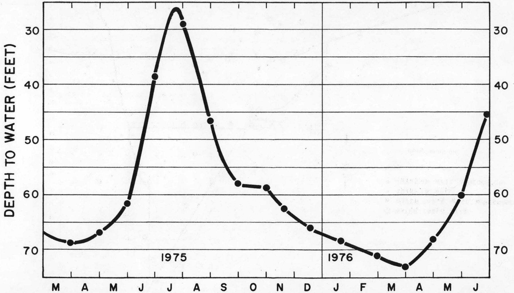
Figure 14. Hydrograph of water table well in the northern part of the Big Wood River-Silver Creek aquifer.
