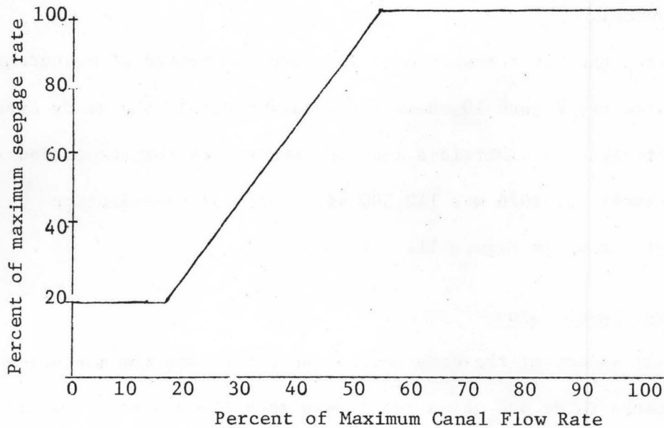
Fig. 9. Variation of canal seepage rate in groundwater model. Big Wood-Silver Creek study.
