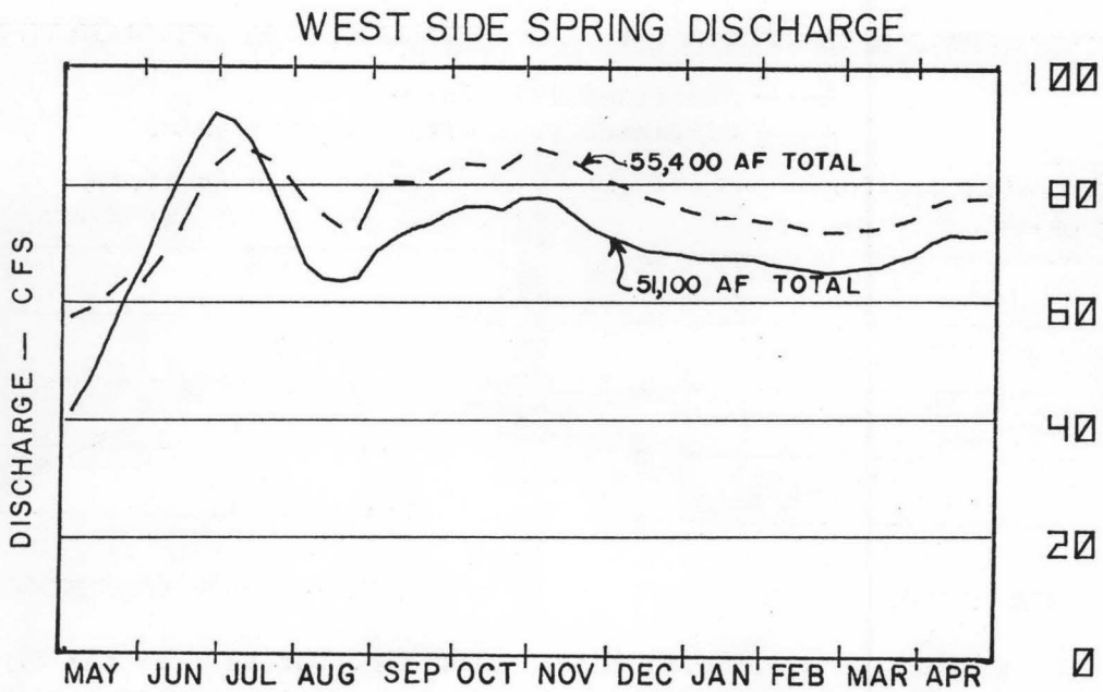
Figure 27. Effects of canal lining on springflows in the Big Wood River-Silver Creek area.
