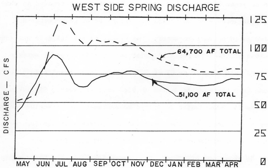
Figure 29. Effects of artificial recharge of flood waters from the Big Wood River on springflows in the Big Wood-Silver Creek area.
