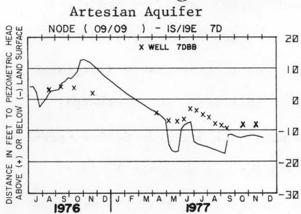
Figure 41. Comparison of simulated groundwater levels and artesian pressures with historical measurements of nearby wells during the 1977 drought in the Big Wood River-Silver Creek area.
