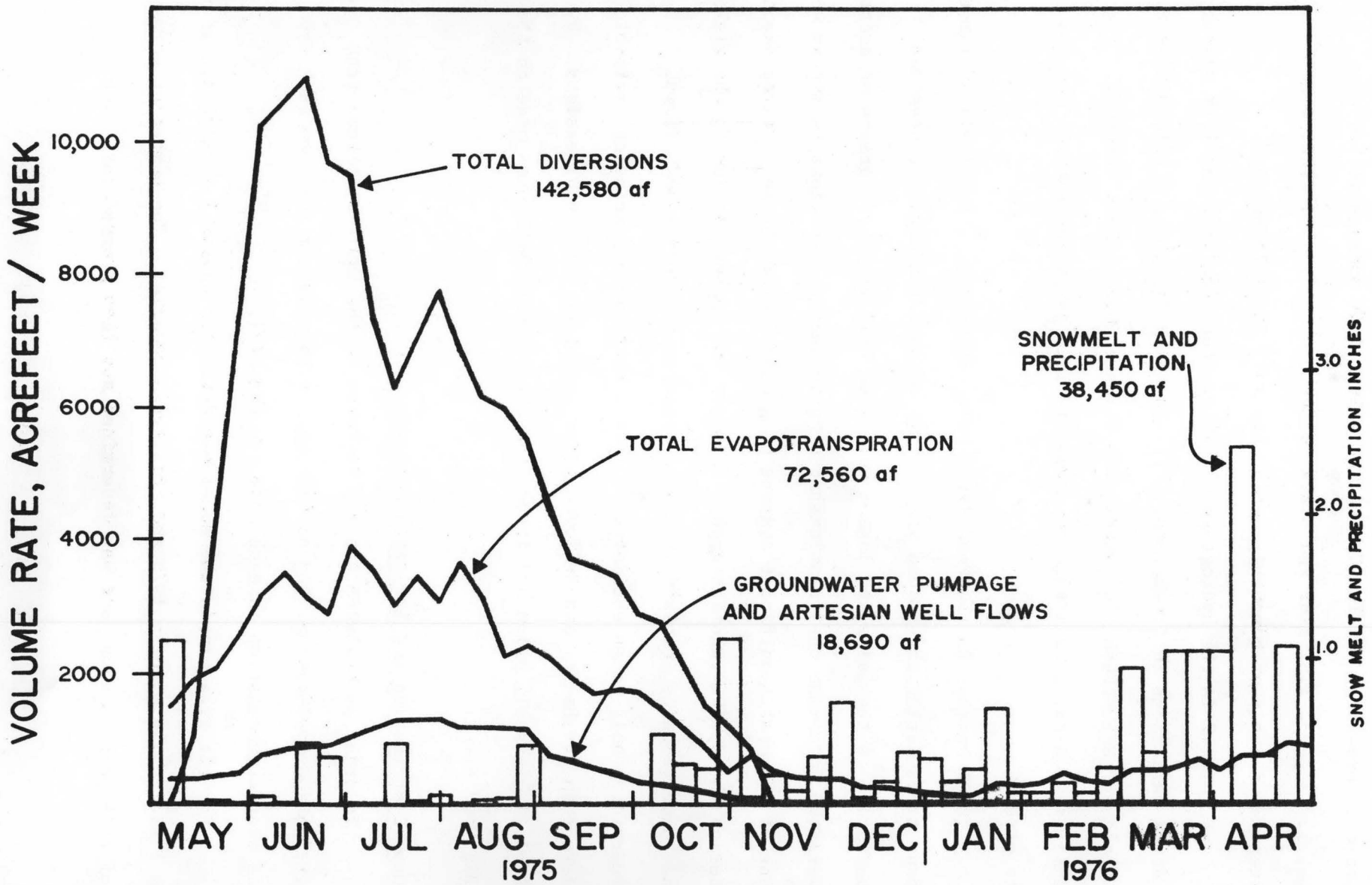
Figure 11. External water budget components. Big Wood River-Silver Creek area. 1975-76
