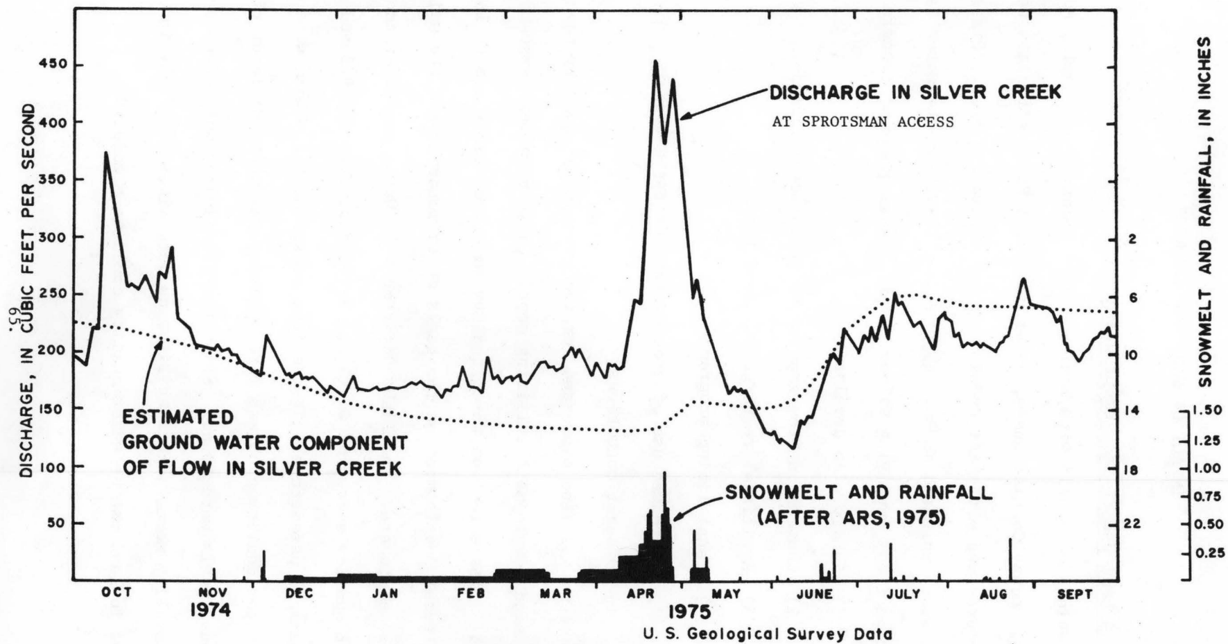
Figure 24. Flow in Silver Creek, groundwater component of flow and snowmelt and rainfall, 1975 water year.
