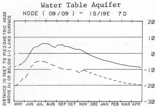
Figure 36. Effects of additional artesian wells on groundwater levels and artesian pressures in the Big Wood River-Silver Creek area.
