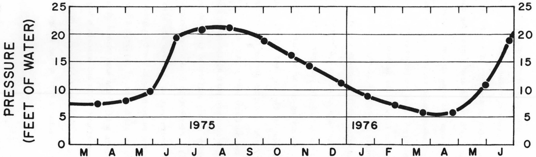
Figure 15. Hydrographs of water table and artesian wells in southern part of Big Wood River-Silver Creek area.
