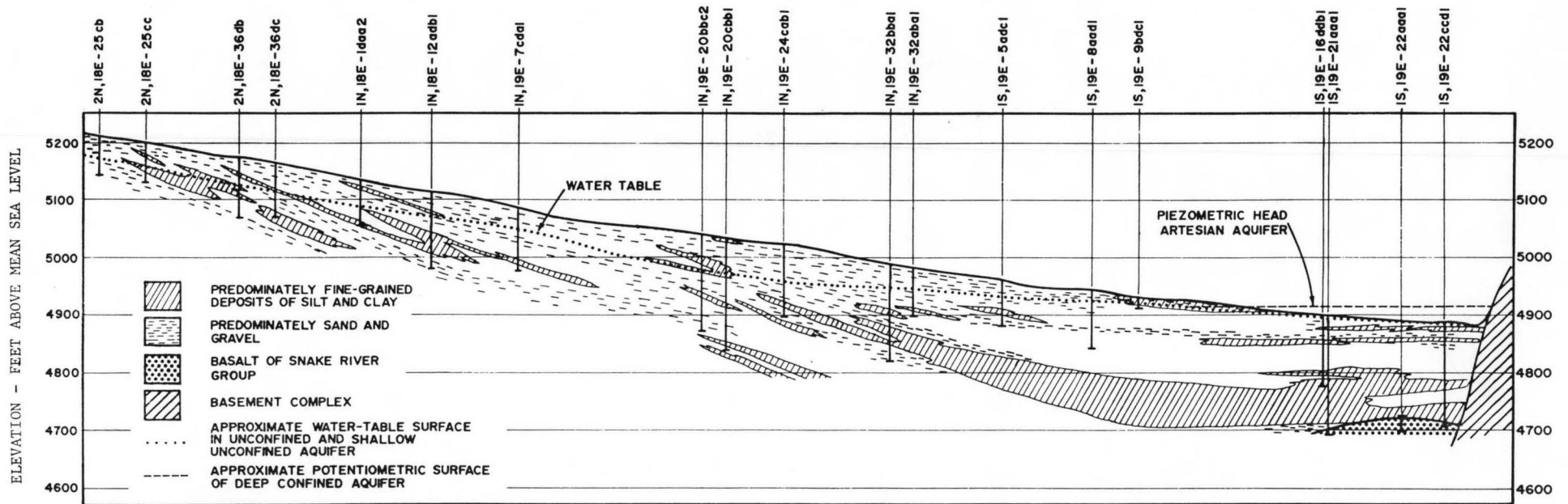
Figure 3. Generalized North to South geologic cross section - Big Wood River - Silver Creek area.
