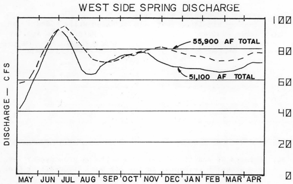
Figure 37. Effects of additional artesian wells on springflows in the Big Wood River-Silver Creek area.
