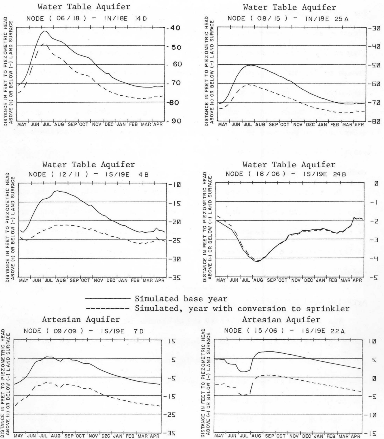
Figure 34. Effects of complete conversion from gravity to sprinkler irrigation in the District 45 Irrigation District on groundwater levels and artesian pressures in the Big Wood River-Silver Creek area.
