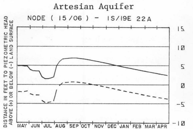
Figure 30. Effects of subdivision development on groundwater levels and artesian pressures in the Big Wood River-Silver Creek area.
