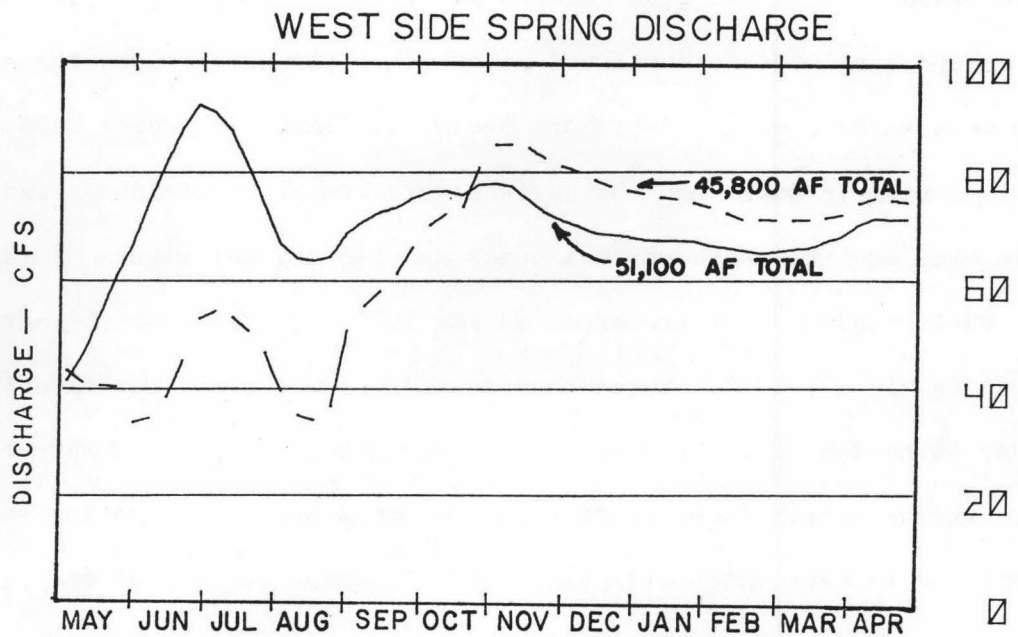
Figure 40. Effects of increased groundwater irrigation development on springflows in the Big Wood River-Silver Creek area.
