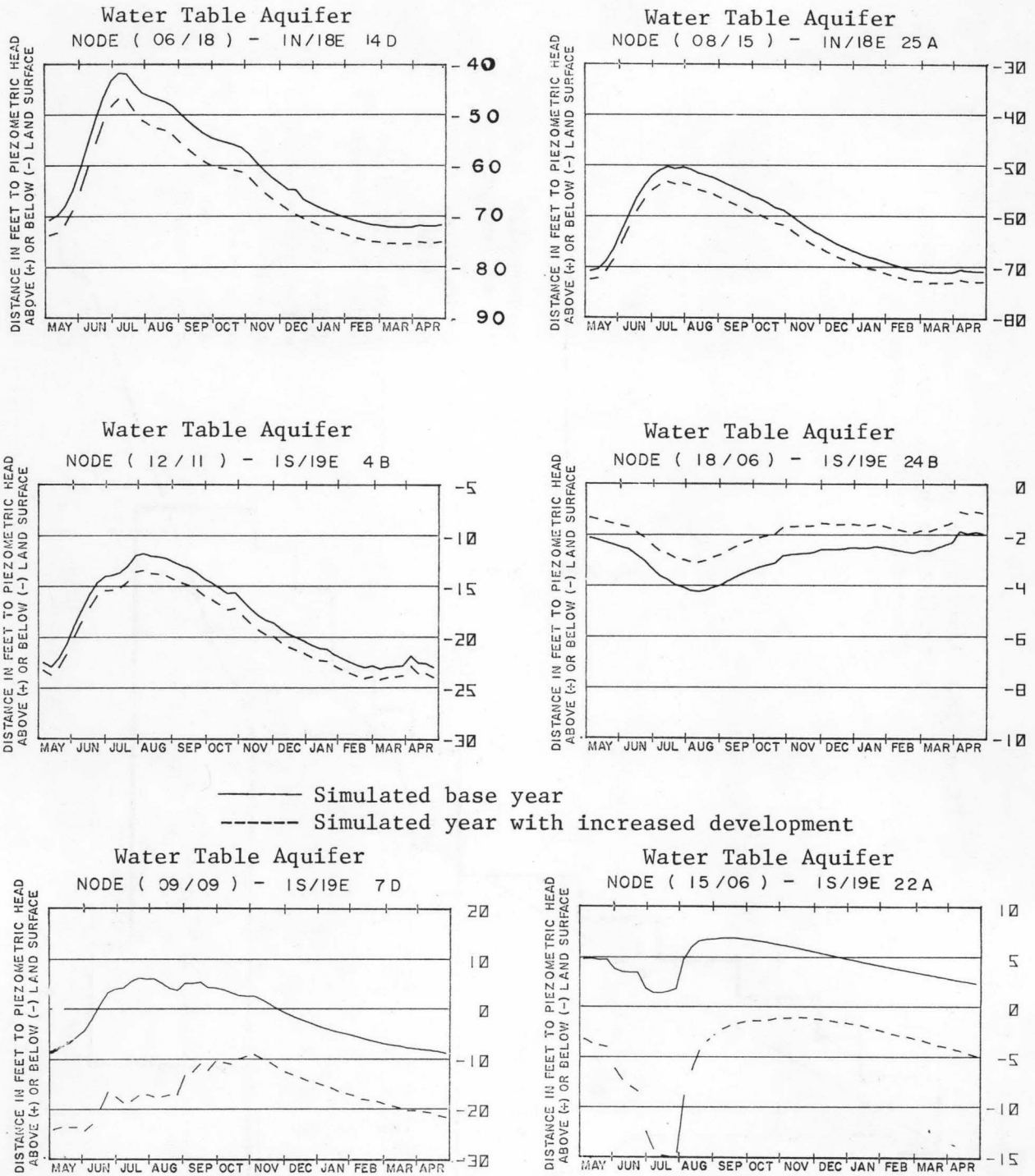
Figure 39. Effects of increased groundwater irrigation development on groundwater levels and artesian pressures in the Big Wood River-Silver Creek area.
