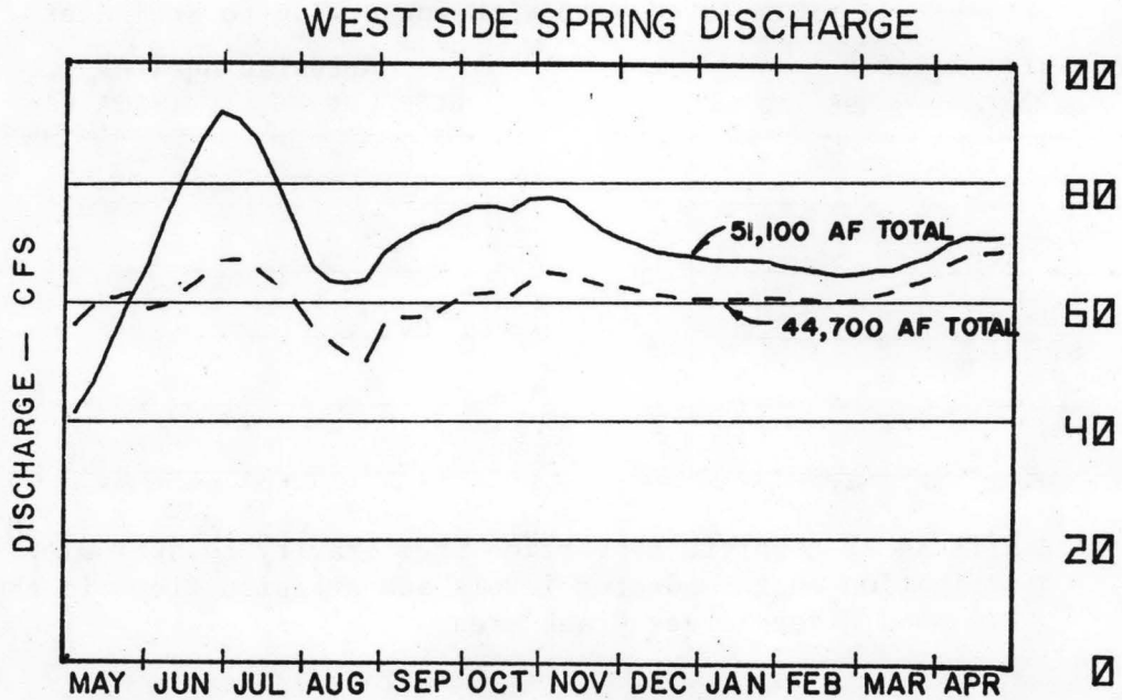
Figure 33. Effects of complete conversion from gravity to sprinkler irrigation on springflows in the Big Wood River-Silver Creek area.
