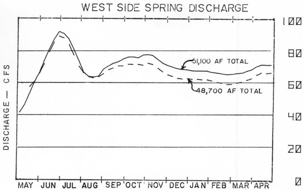
Figure 23. Comparison of simulated springflows with historical flow measurements in the Big Wood River-Silver Creek area.
