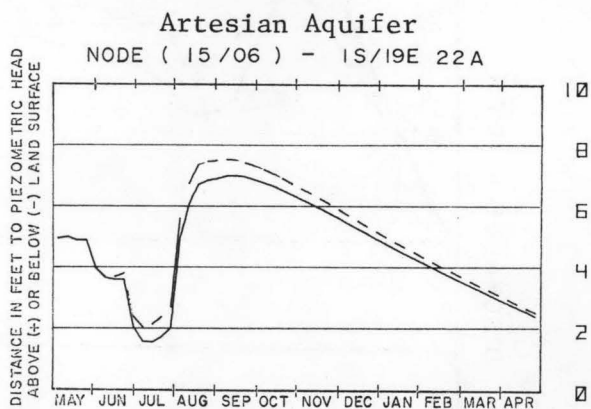
Figure 28. Effects of artificial recharge of floodwaters from the Big Wood River on groundwater levels and artesian pressures in the Big Wood-Silver Creek area.
