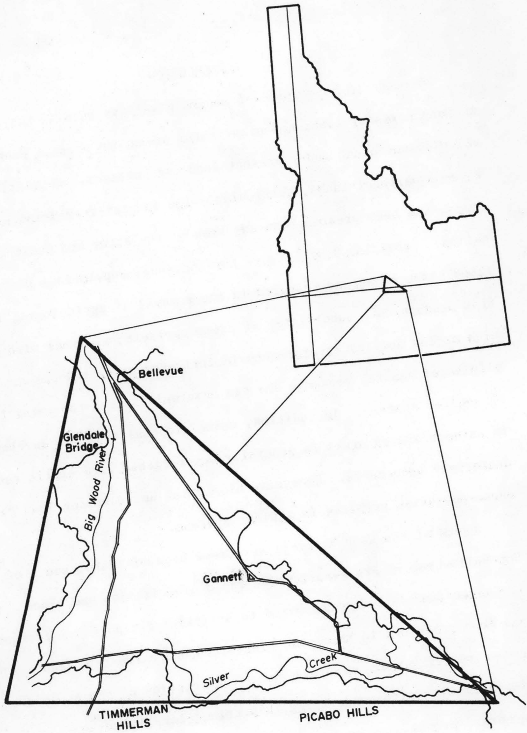
Figure 1. Location map - Big Wood River-Silver Creek area, Idaho
