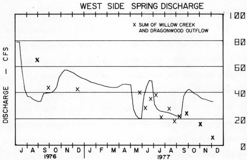
Figure 42. Comparison of simulated springflows with historical flow measurements during the 1977 drought in the Big Wood River-Silver Creek area.
