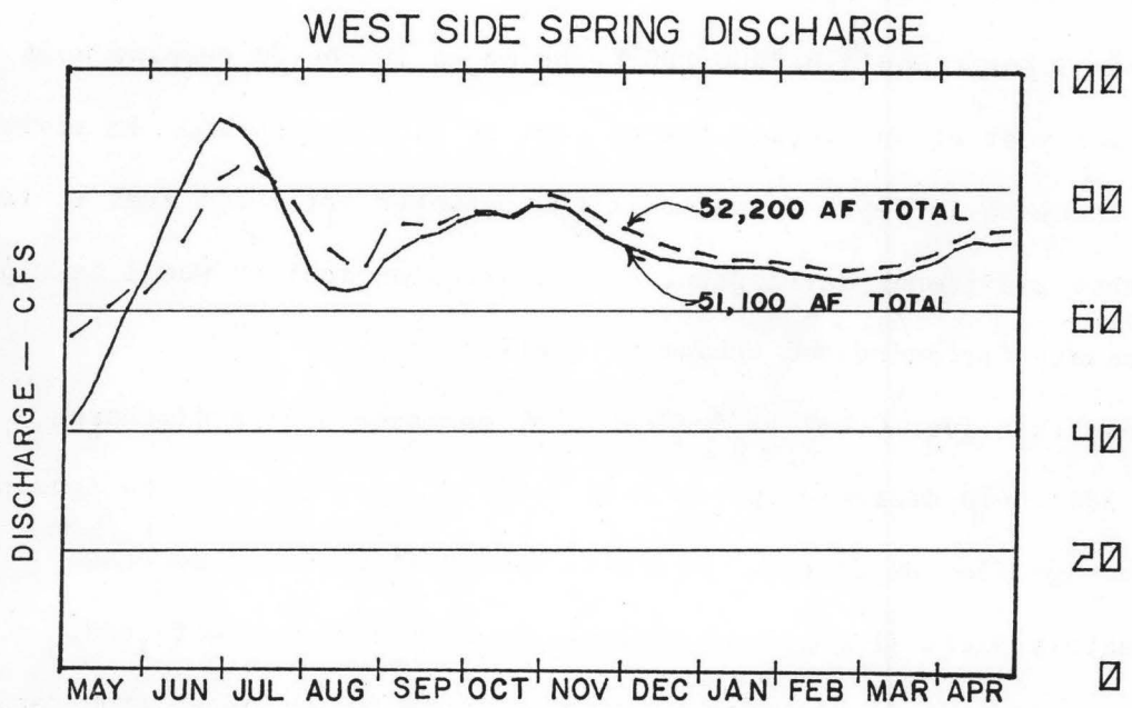
Figure 31. Effects of subdivisions development on springflows in the Big Wood River-Silver Creek area.
