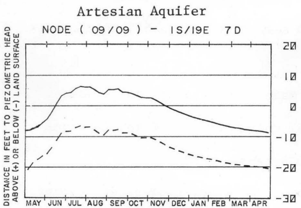
Figure 30. Effects of subdivision development on groundwater levels and artesian pressures in the Big Wood River-Silver Creek area.
