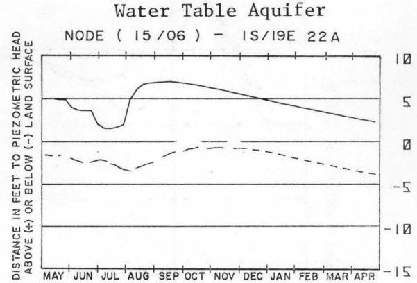
Figure 36. Effects of additional artesian wells on groundwater levels and artesian pressures in the Big Wood River-Silver Creek area.
