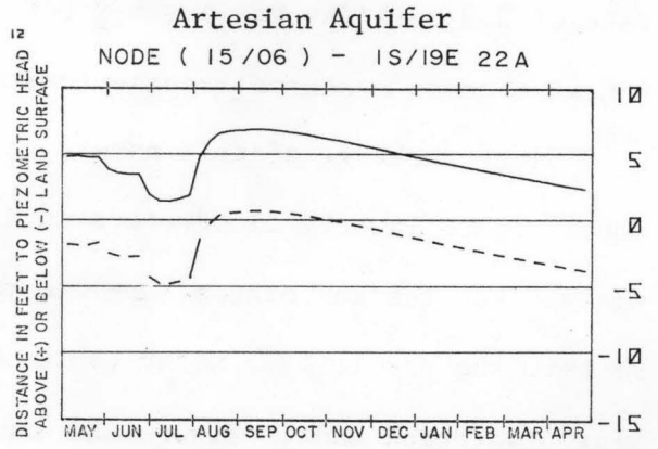
Figure 26. Effects of canal lining on groundwater levels and artesian pressures in the Big Wood River-Silver Creek area.
