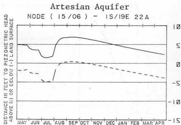
Figure 32. Effects of complete conversion from gravity to sprinkler irrigation on groundwater levels and artesian flows in the Big Wood River-Silver Creek area.
