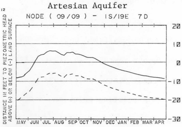
Figure 26. Effects of canal lining on groundwater levels and artesian pressures in the Big Wood River-Silver Creek area.
