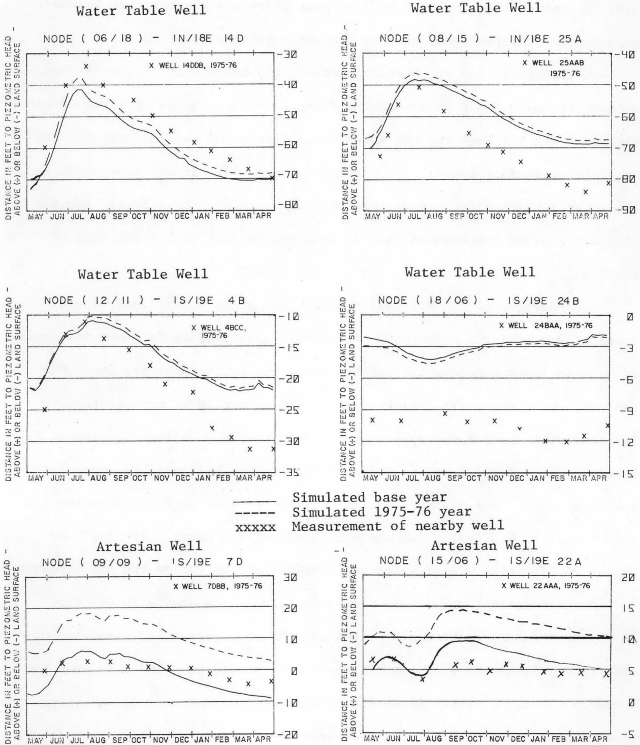
Figure 22. Comparison of simulated groundwater levels and artesian pressures with historical measurements of nearby wells in the Big Wood River-Silver Creek area.
