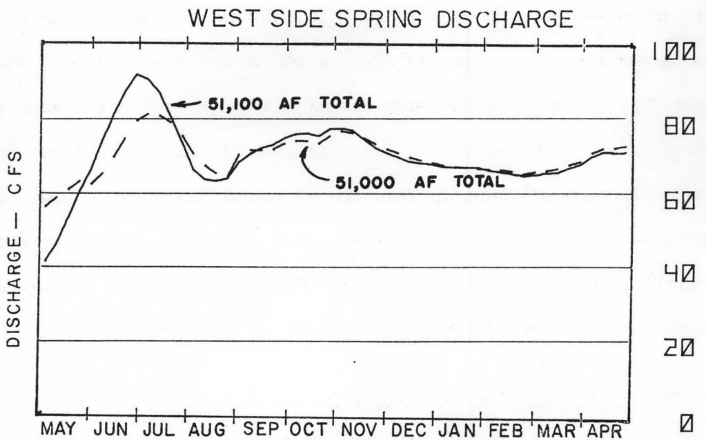
Figure 35. Effects of complete conversion from gravity to sprinkler irrigation in the District 45 Irrigation District on springflows in the Big Wood River-Silver Creek area.
