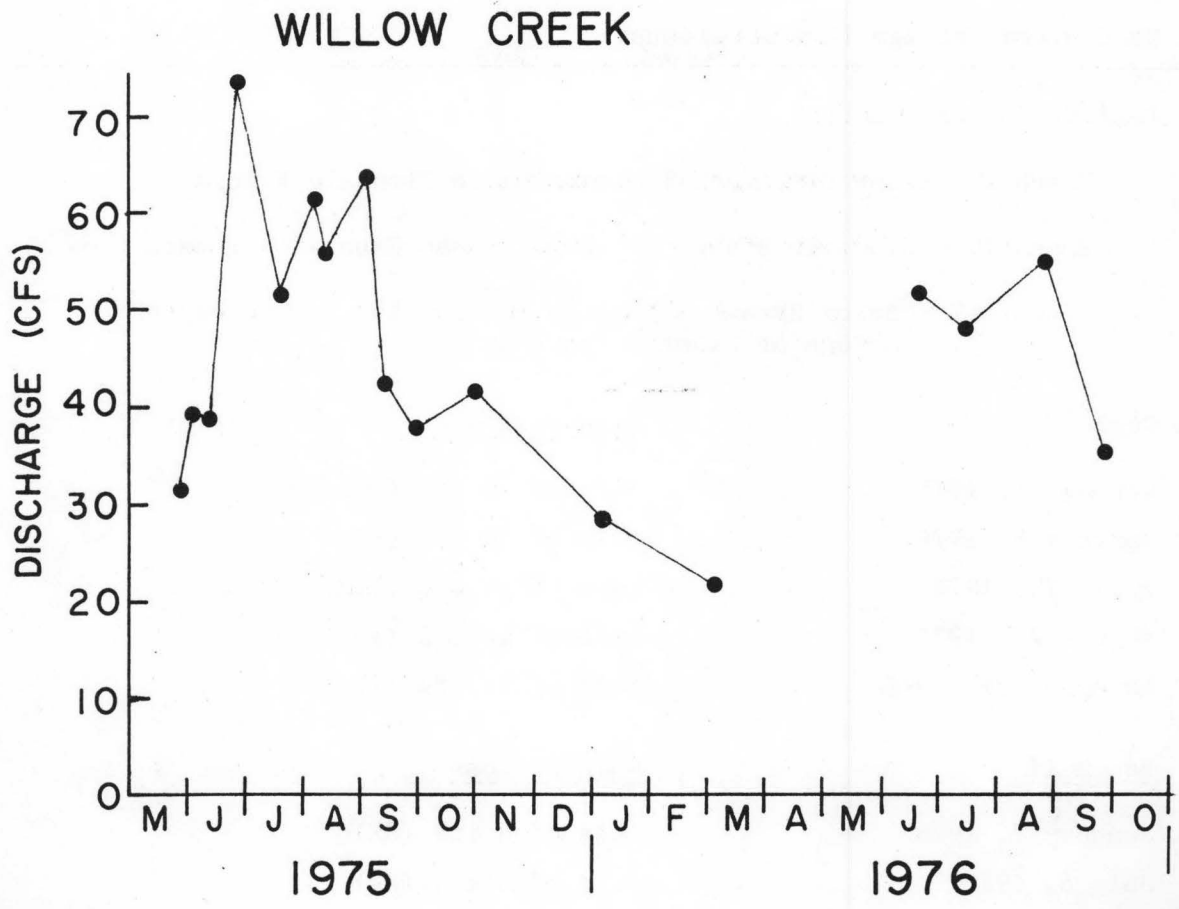
Figure 12. Hydrograph of Willow Creek Big Wood River-Silver Creek area, 1975-76
