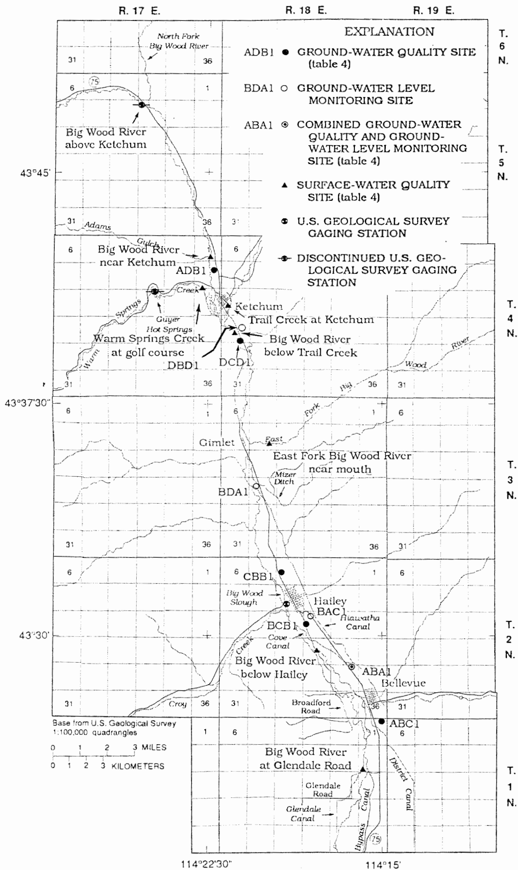
Figure 10.--Locations of water-quality and ground-water level monitoring sites.
