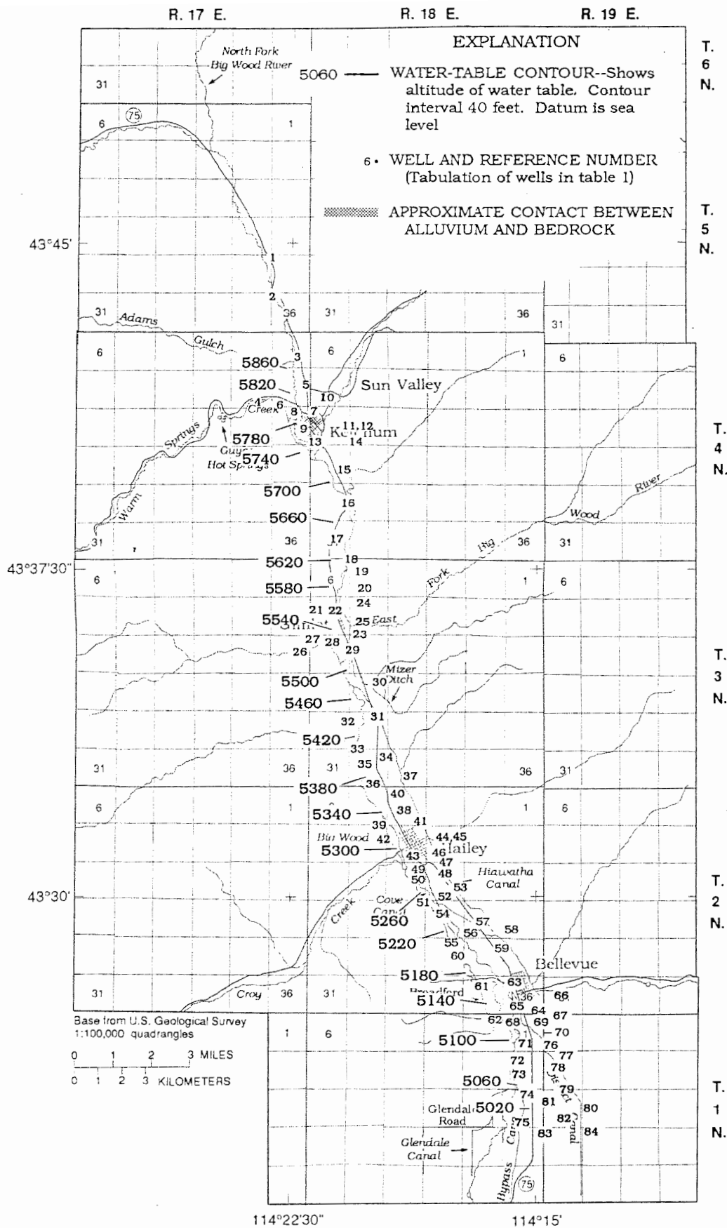
Figure 7.--Water-table contours in April 1986 and well locations
