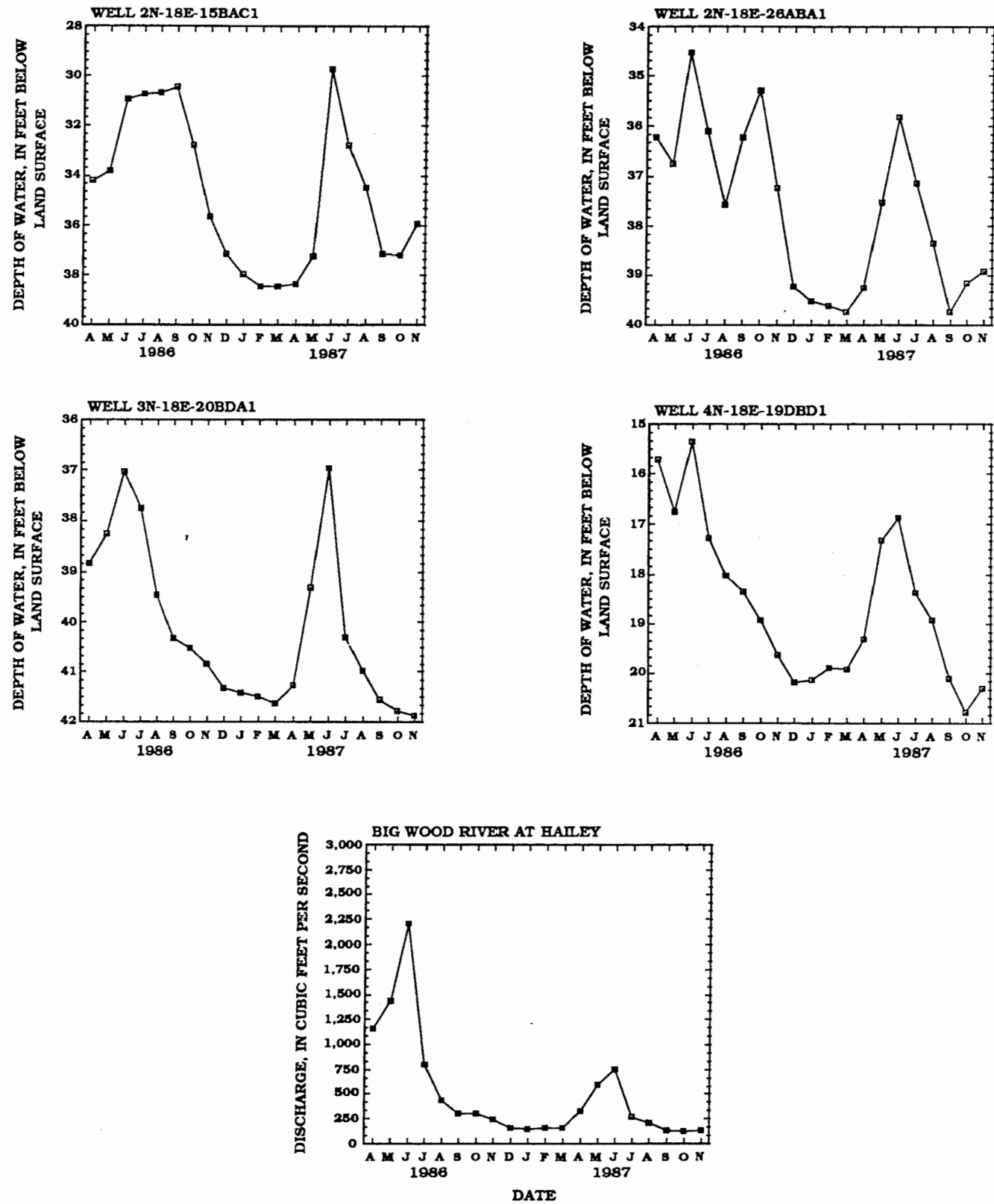
Figure 9.--Water levels for selected observation wells and discharge of the Big Wood River at Hailey. (Locations shown in figure 10)
